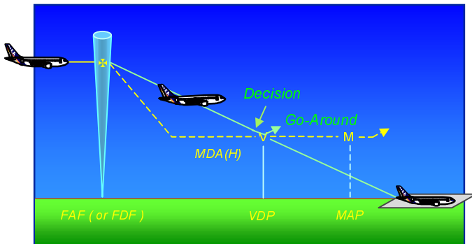
Figure 3 Constant-angle Final Approach
