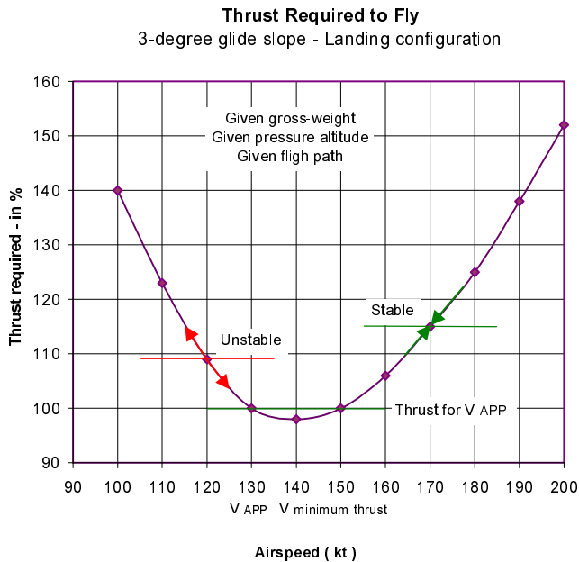
Figure 2 Power Curve - Typical
