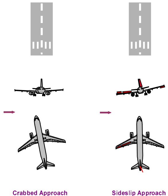
Figure 1 Crabbed Approach versus Sideslip Approach
