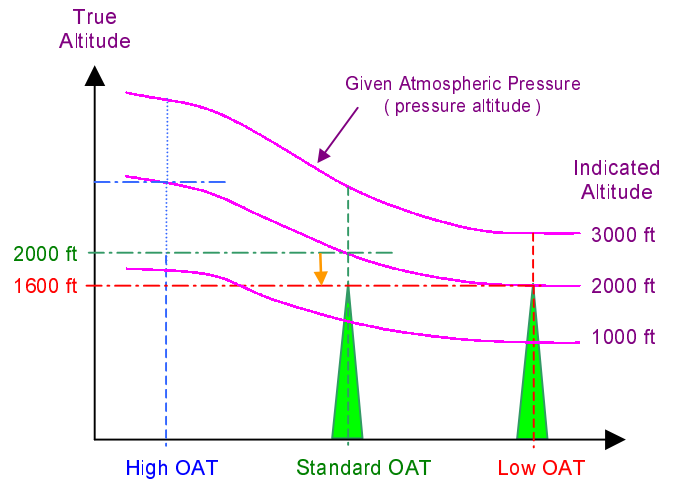
Figure 1 Effect of OAT on True Altitude
