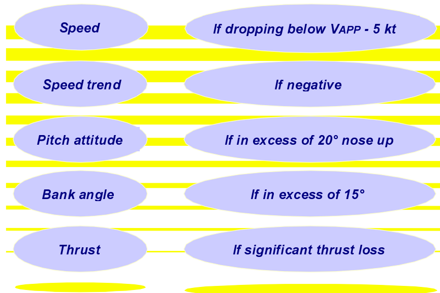
Figure 1 Excessive Deviation Callouts in Go-around
