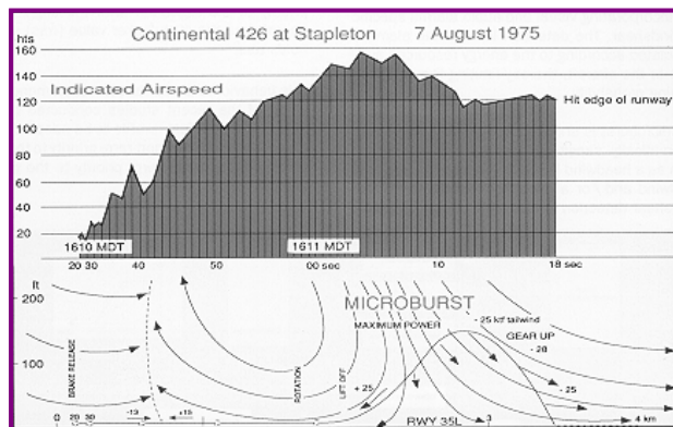
Figure 1 Wind Shear Profile - Typical
