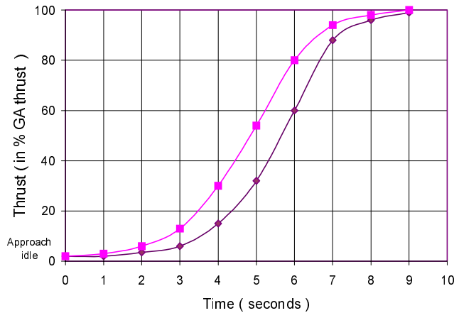
Thrust Response from Idle to GA Thrust ( typical engine-to-engine scatter )
