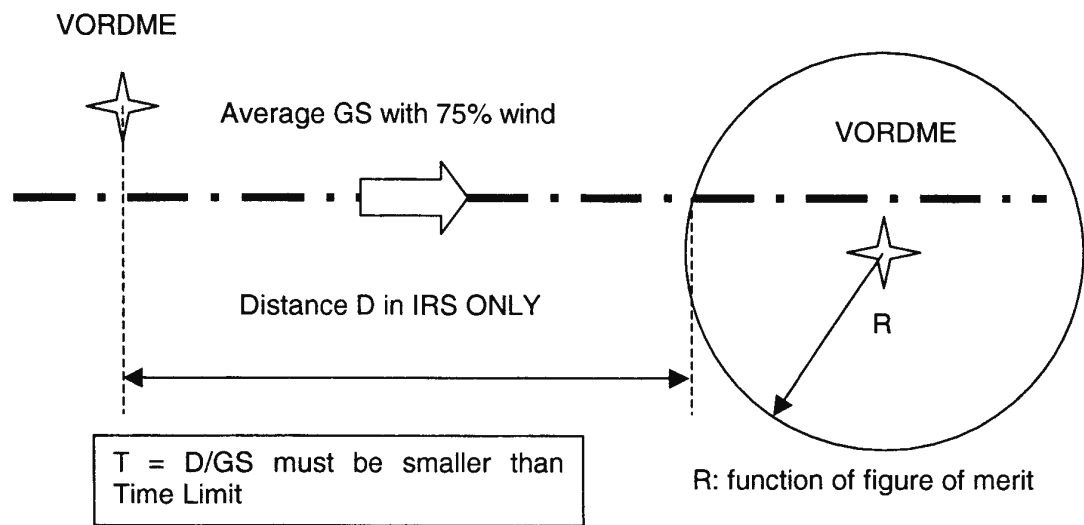
Figure 4 : Estimation of flight length in IRS ONLY navigation
